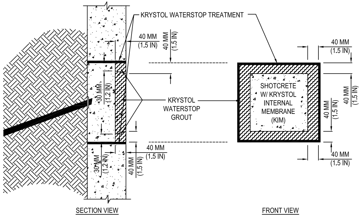
SHOTCRETE: TIE BACK BLOCKOUT DOUBLE PROTECTION; EXTERNAL GROUT METHOD
